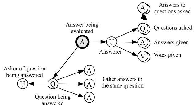
Figure 3: Types of features available for inferring the quality of an answer.
