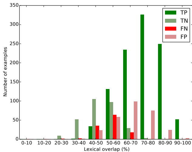
Figure 3: Results for the ‘OoB + both aux – unwghd + swsn’ run, grouped by percentage of lexical overlap between test sentences in the MSR Paraphrase Corpus. (Best viewed in color.)
