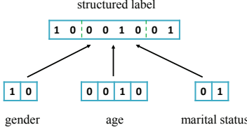
Figure 2: Structured representation of multi-task multi-class predictions.
